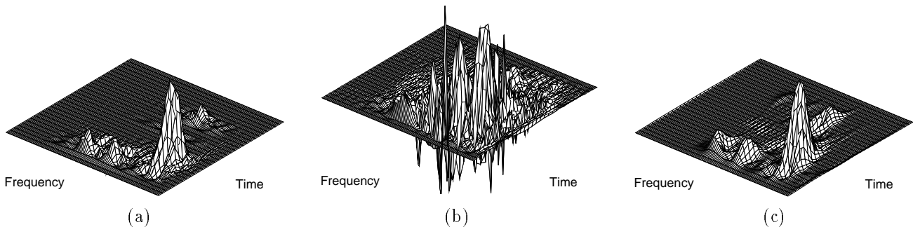
Figure 4. Mesh plots for the signal g(t) : (a) SIAP-LTD based time-frequency distribution; (b) Wigner distribution; (c) Smoothed pseudo Wigner distribution. The SIAP-LTD yields an adaptive distribution where high resolution, high concentration, and suppressed cross-term interference are attainable.
