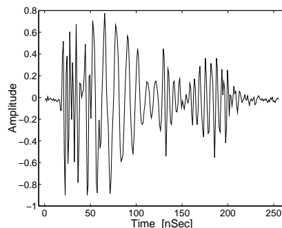
Figure 1. The signal g(t) : Evolution of an electromagnetic pulse in a relativistic magnetron (heterodyne detection; local oscillator=2.6GHz).
